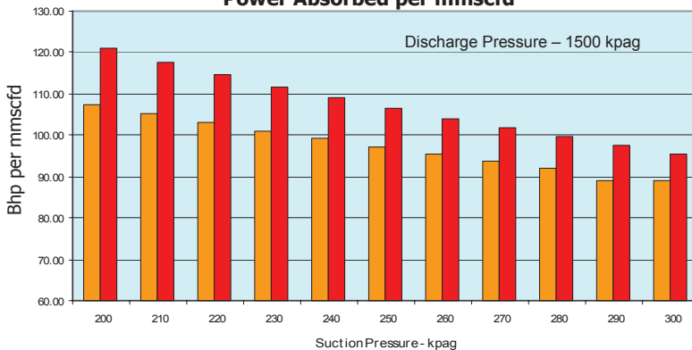
AJAX DPC3404 vs Screw Compressor Power Absorbed per mmscfd
